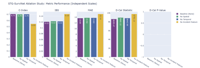
Figure 8. STG-SurviNet Ablation Study: Metric Performance (Independent Scale)
